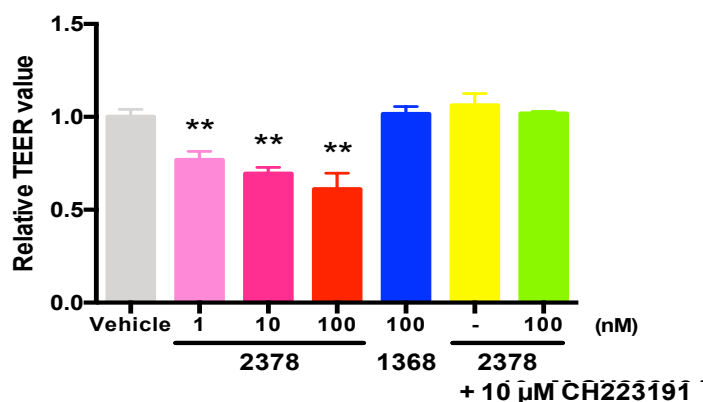
Fig. 2 Effects of TCDD on TJ barrier in Caco-2 cells.
