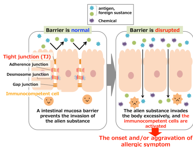
Fig. 1 Biogenic defense mechanism of intestinal mucosa barrier.
