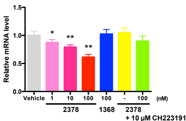
Fig. 4 Expression of claudin-4 in Caco-2 cells treated with TCDD.
