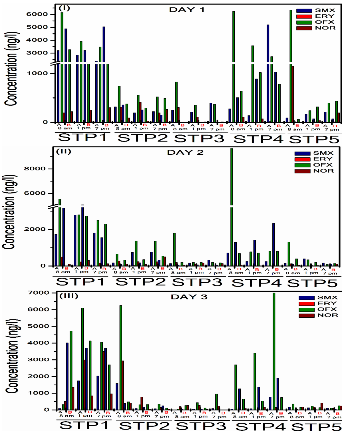
Fig.1. (I) Concentrations antibiotics of Day 1; (II) Concentrations antibiotics of Day 2; (III) Concentrations antibiotics of Day 3; at three-time intervals in five STPs; A: inlet; B: outlet SMX: Sulfamethoxazole; ERY: Erythromycin; OFX: Ofloxacin; NOR: Norfloxacin
