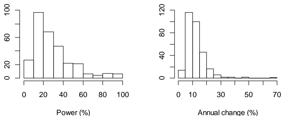
Figure 5. Based on the results of 316 legacy POP time-series. Left: Frequency of the power (%) to detect a 5% annual change in a 10 years period with a sign. level of 5%. Right: Frequency of lowest detectable trend in a 10 year period with a power of 80% and sign. level of 5%. Redrawn from. 10
