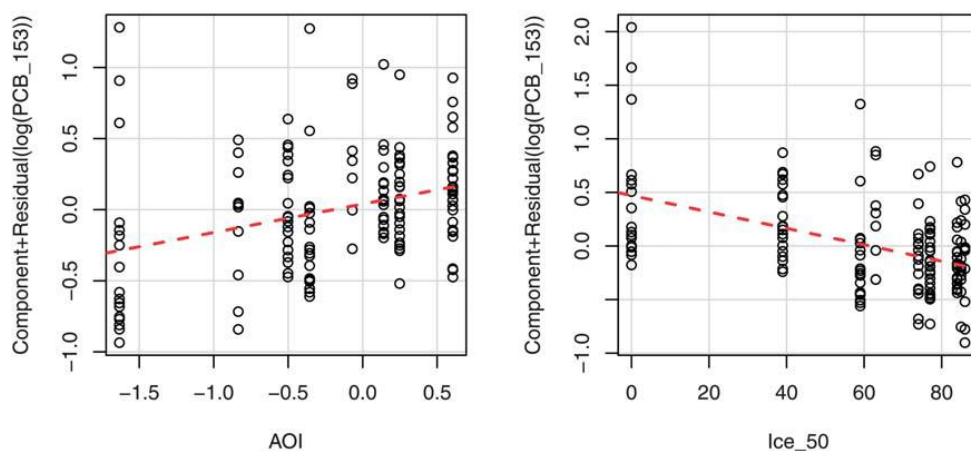
Figure 6. Component-residual plots show the relationships between PCB-153 concentrations in ringed seal blubber from central West Greenland and the winter Arctic Oscillation Index (AOI) (left) and number of days with ice coverage above 50% during winter (Ice_50) (right). Redrawn from. 3
