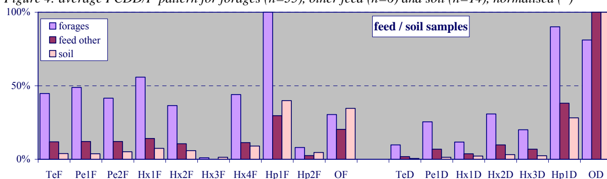
Figure 4: average PCDD/F-pattern for forages (n=35), other feed (n=6) and soil (n=14), normalised (*)
