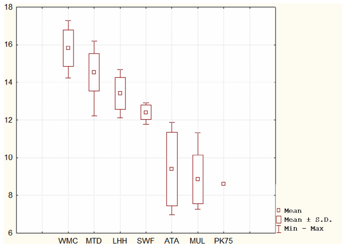
Fig.1. Delta ^{15}\text{N} values in species of the Guanabara Bay food web (WMC, whitemouth croaker; MTD, marine tucuxi dolphin; LHH, largehead hairtail; SWF, smooth weakfish; ATA, Atlantic anchoveta; MUL, mullet; PK75, seston samples collected using a 75-nm-mesh plankton net).
