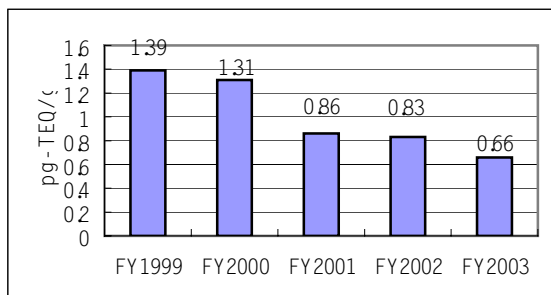
Figure 2 Trend of Dioxin concentrations in Pine needles
