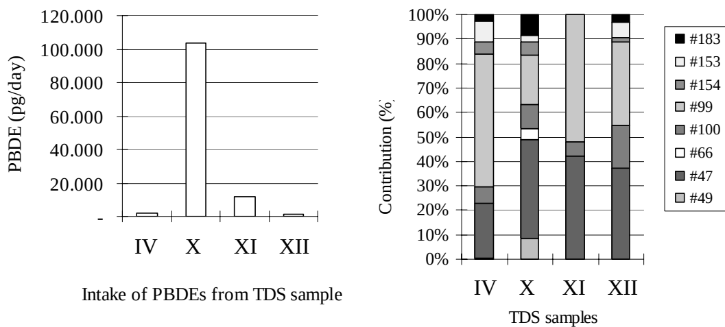
Fig.3 Daily intake and congener profiles of PBDEs in the TDS samples
