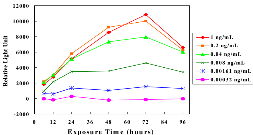
Figure 1 Effect of 2378-TCDD exposure duration on the luminescence of H4IIE-luciferase cells in vitro at various dose levels are expressed as the concentration in microplate wells.
