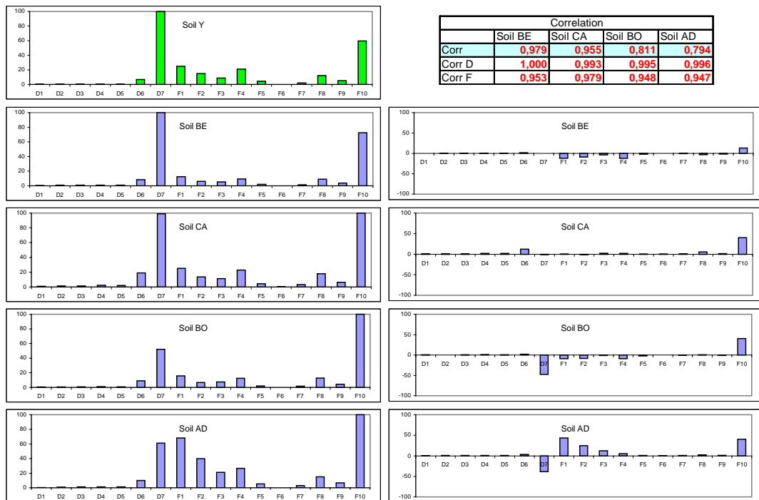
Figure 2: PCCD+PCDF profiles of the five soil samples. In the table are reported the Pearson correlation coefficients for the dioxins (Corr.D) and for the furans (Corr.F), calculated with respect to profile of the Y sample. In the left side are shown the profiles of the five samples, in the right side are shown the profile differences among each profile and the Y sample, the lowest contaminated one.
