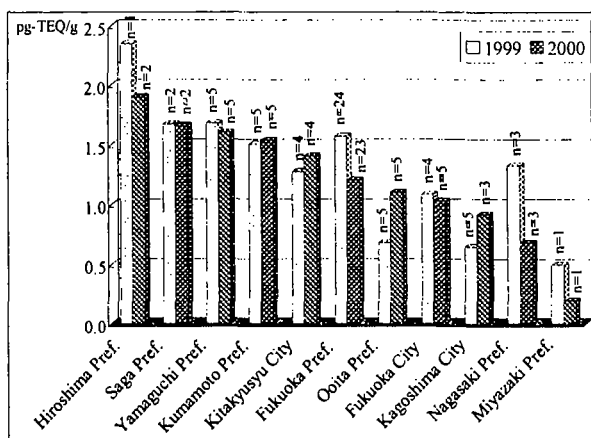
Figure 1 D/F concentration of prefectural average in 1999 and 2000 Unit: pg-TEQ/g
