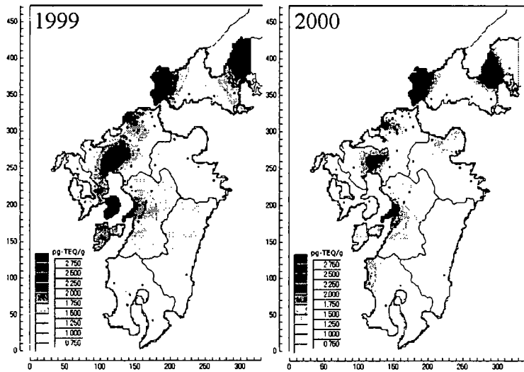
Fig.3 Pine needle D/F concentration in west Japan at municipal levels in 1999 and 2000 unit: pg-TEQ/g
