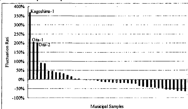
Figure.2 Fluctuation ratio of the D/F Concentration in Pines in 1999 and 2000 in West Japan Area (42 municipal or area wide average samples)
