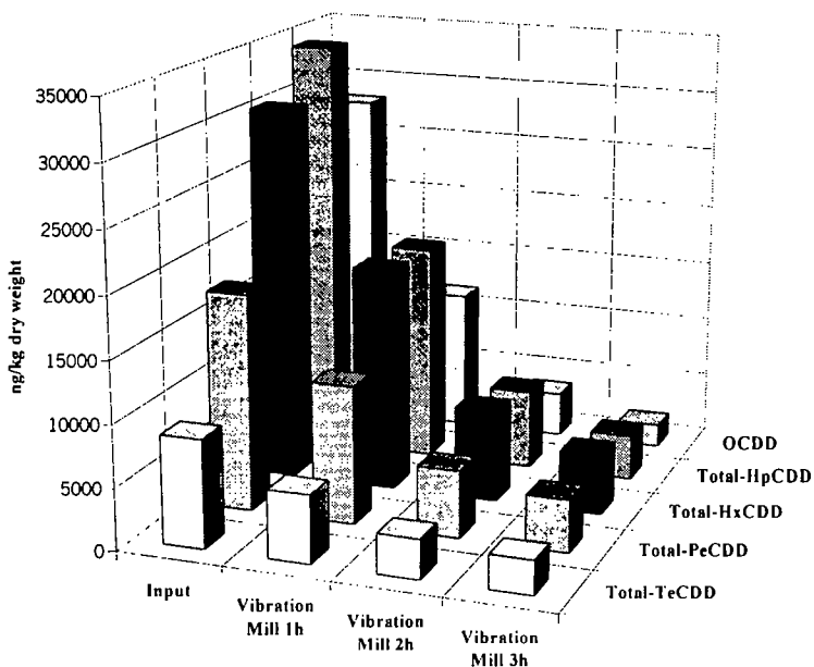
Figure 2: Decrease of concentration of PCDD depending on the period of grinding in a vibratory mill.
