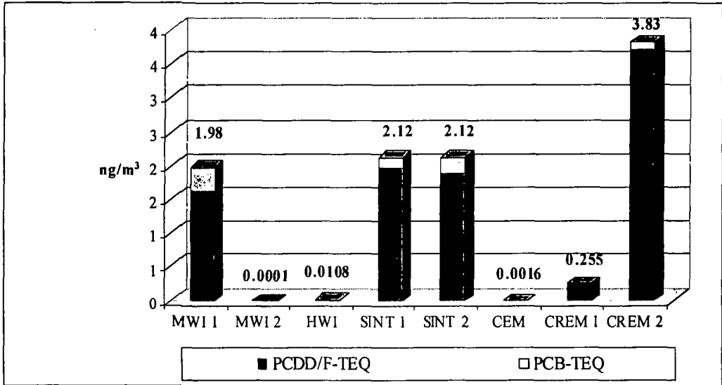
Fig. 01: Total TEQ emissions of industrial sources
