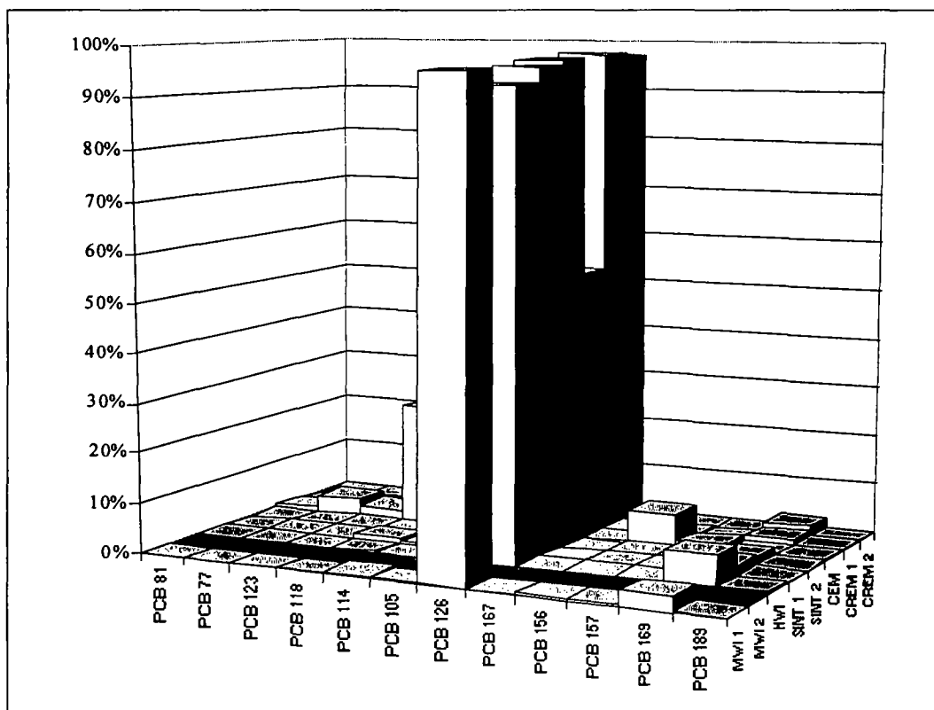
Fig. 04: Proportional contribution of individual PCBs to the PCB-TEQ
