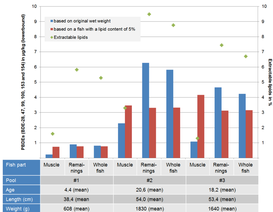
Figure 4: PBDEs in bream – Comparison between different parts of the fish
